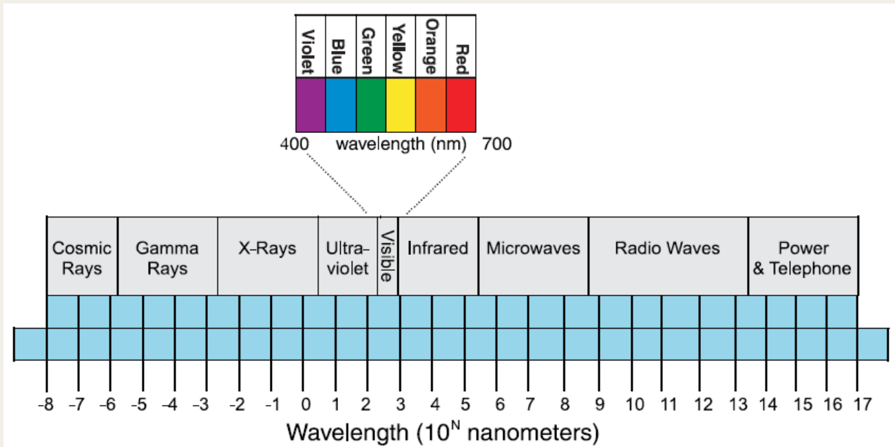
Graph 1: Electromagnetic Spectrum
