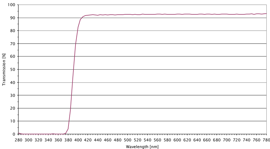
Spectral transmittance ACRYLITE® Film 0F008, thickness = 53 µm
