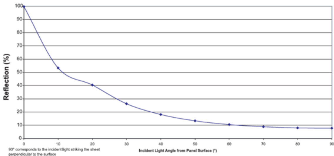
Figure 2) Reflection of ACRYLITE® Soundstop sheet
